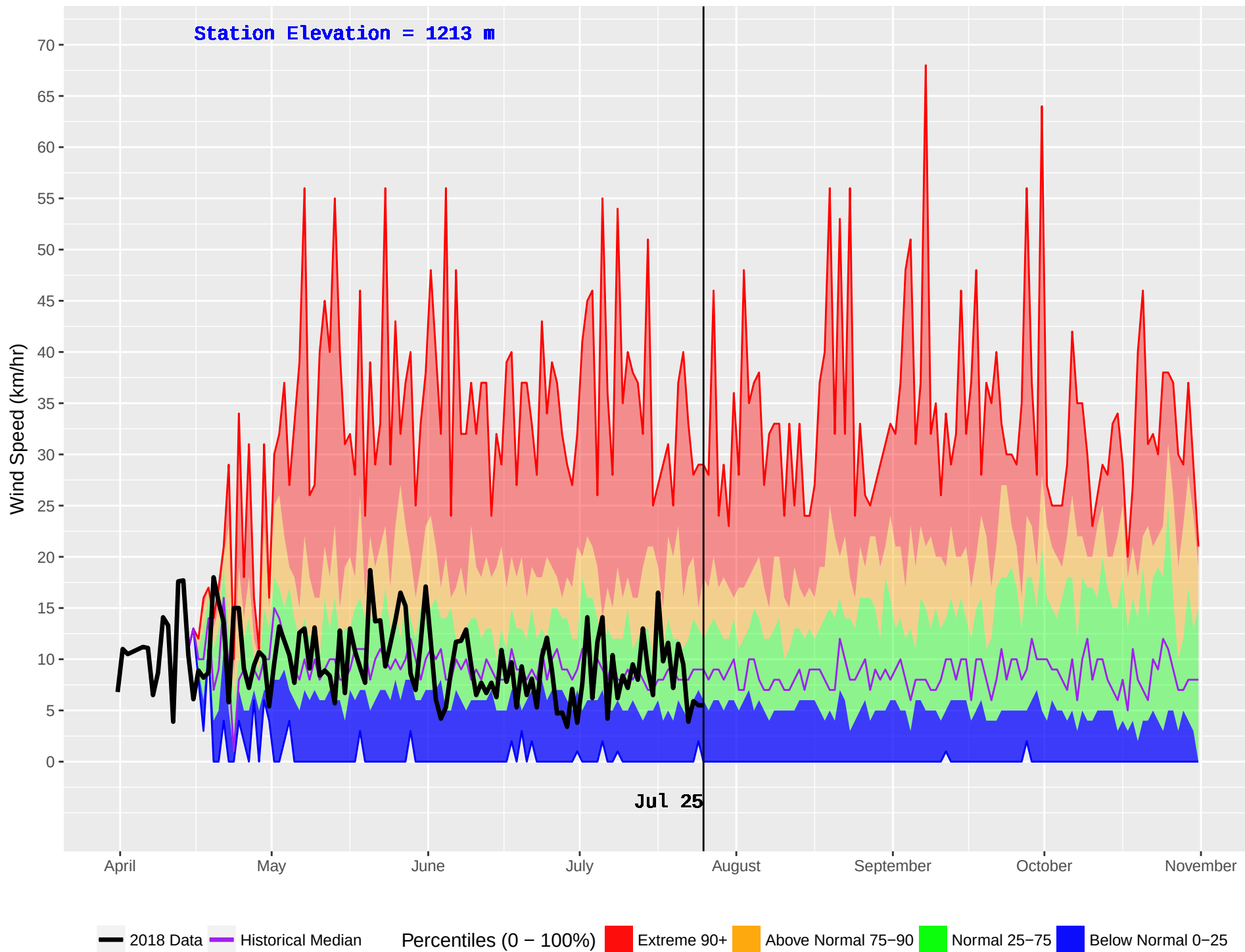
INGENIKA POINT (145) : Historical (1971–2016) and Current (2018) Noon Wind Speed
